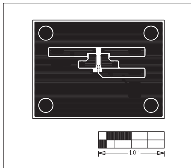
Figure 3. MAX9938 EV Kit PCB Layout—Component Side
