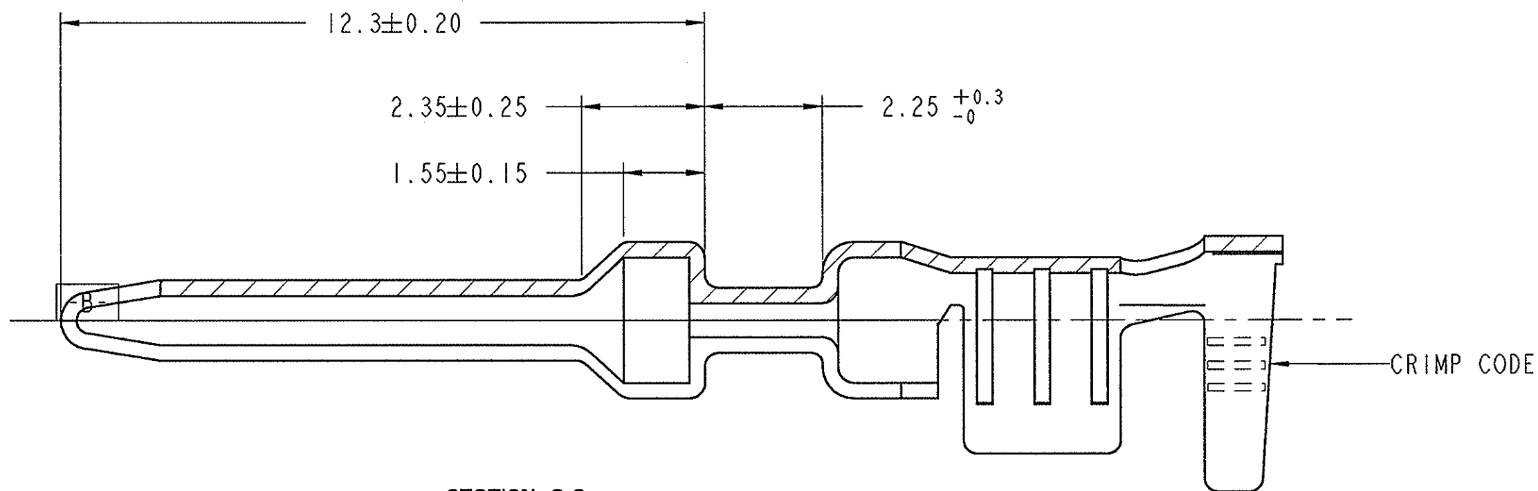
SECTION C-C
