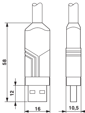
Dimensional drawing
