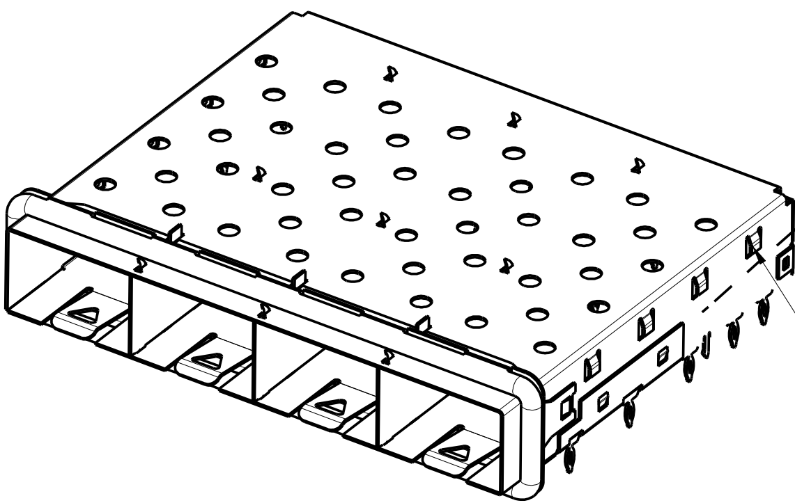
SFP PLUS 1X4 CAGE ASSEMBLY
