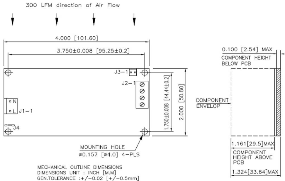
Figure 2 - Mechanical Drawing
