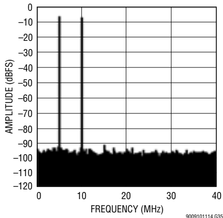
LTM9009-14: 8k Point 2-Tone FFT, f_{IN} = 70\text{MHz} , 75\text{MHz} , -7\text{dBFS} per Tone, 80\text{Mpsps}
