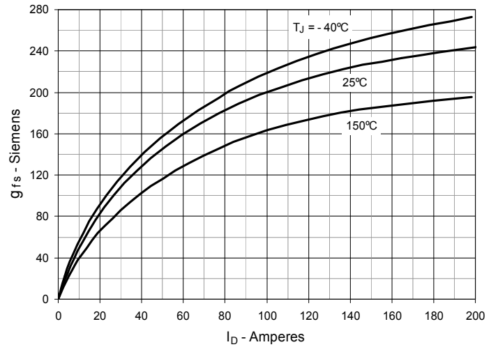
Fig. 8. Transconductance
