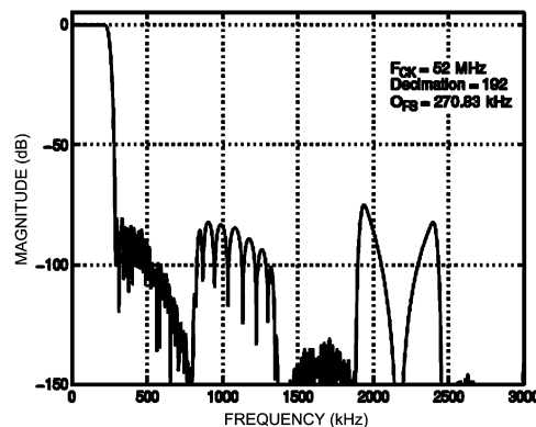
Figure 70. CIC, F1, & F2 STD frequency response
