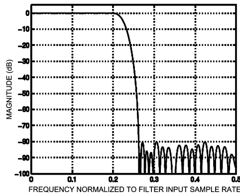
Figure 68. F2 STD frequency response
