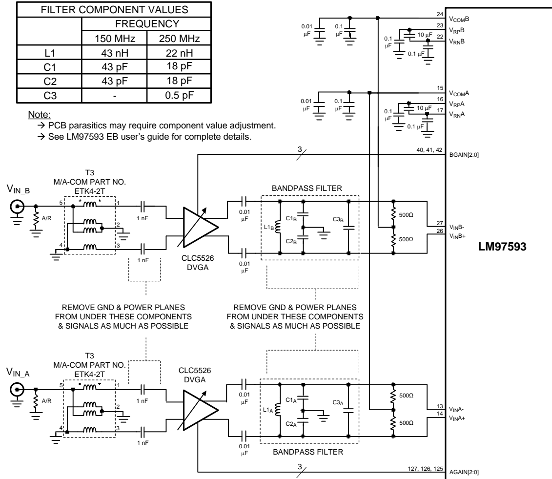
Figure 86. Application Circuit
