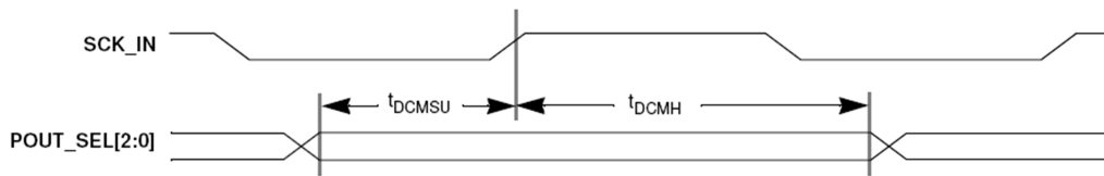
Figure 8. LM97593 Dual Chip Mode Timing
