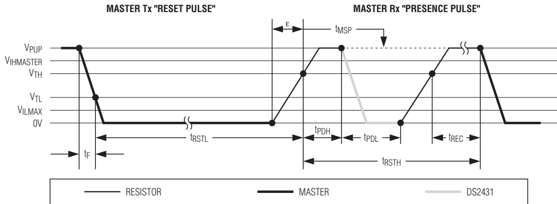
Figure 10. Initialization Procedure: Reset and Presence Pulse
