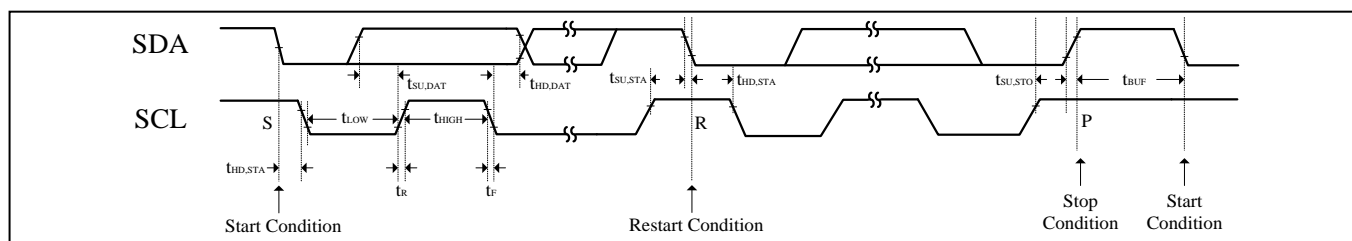
Figure 2 Interface timing
