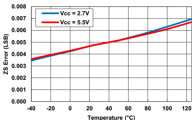
Figure 6. ZS Error vs Temperature for 10kΩ
