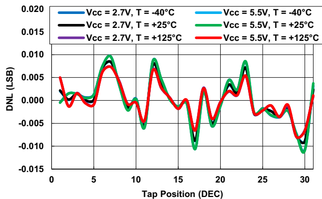
Figure 4. DNL vs Tap Position in Voltage Divider Mode for 10kΩ
