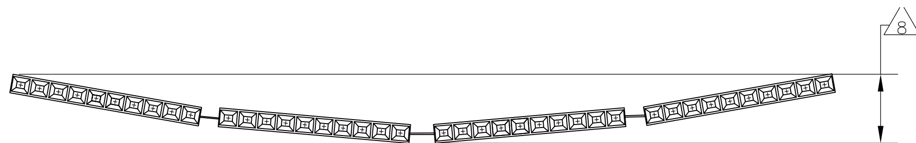
CONTACTS ARE LATCHED INTO THE PRELOAD WINDOWS USE WITH #22-#26 AWG WIRE SIZE, .054/.030 INSULATION DIAMETER, .015 MAXIMUM INSULATION THICKNESS THE DIMENSION APPLIES WITH THE FORWARD PRELOAD STOP IN CONTACT WITH THE HOUSING SURFACE POINT OF MEASUREMENT FOR PLATING THICKNESS FOR INDIVIDUAL ASSEMBLIES SEE PART NUMBER 103687 ASSEMBLIES ARE JOINED BY THE CARRIER STRIP. ORDER QUANTITY REFLECTS TOTAL NUMBER OF INDIVIDUAL ASSEMBLIES REQUIRED . SEE TABLE FOR NUMBER OF ASSEMBLIES PER STRIP. POINT OF MEASUREMENT FOR PLATING THICKNESS (INSIDE BEAMS) MAXIMUM ALLOWABLE BOW OF ASSEMBLY NOT TO EXCEED .055. CONTACTS: .000100-.000200 BRIGHT TIN-LEAD OVER .000050 NICKEL. CONTACTS: .000100-.000200 MATTE TIN OVER .000050 NICKEL.
