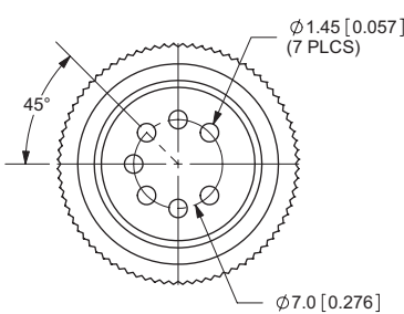
SD-70LP
