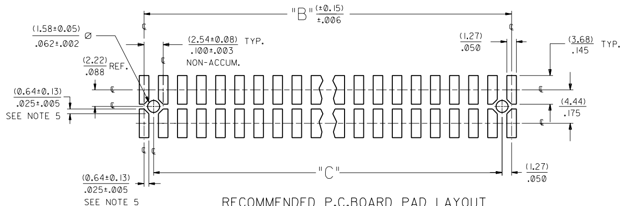
RECOMMENDED P.C.BOARD PAD LAYOUT
