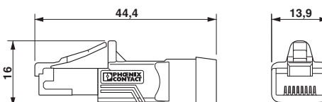
Dimensional drawing
