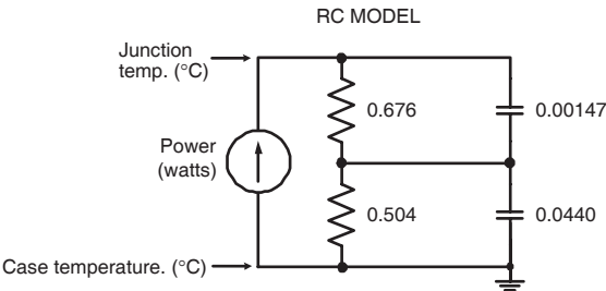
FIGURE 25b. TRANSIENT THERMAL IMPEDANCE MODEL
