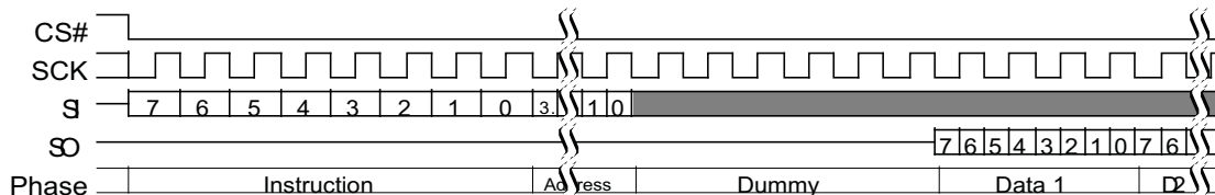
Figure 90. DDR Fast Read Subsequent Access (4-Byte Address, HPLC=01b)
