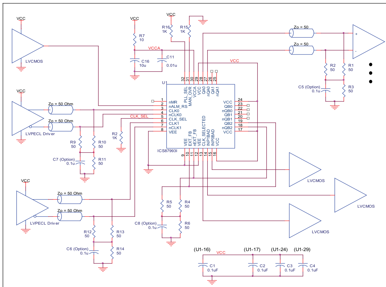
FIGURE 5A. 87993I LVPECL SCHEMATIC EXAMPLE
