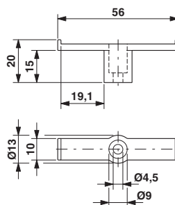
Dimensional drawing
