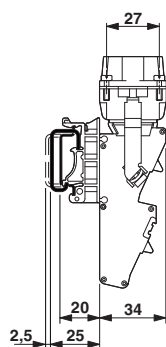
Dimensional drawing
