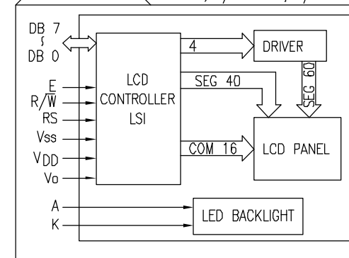
BLOCK DIAGRAM 20 x 2, 1/16 DUTY, 1/5 BIAS
