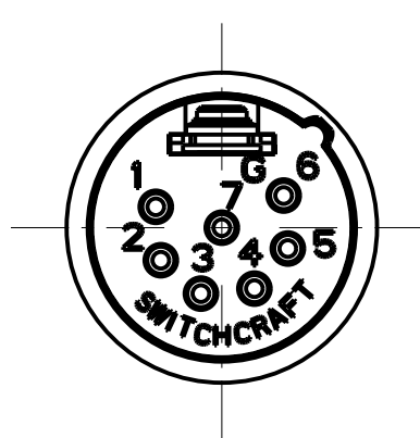
7 PIN
