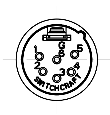
6 PIN
