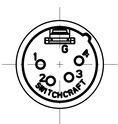
4 PIN
