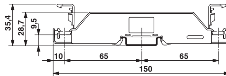
Dimensional drawing
