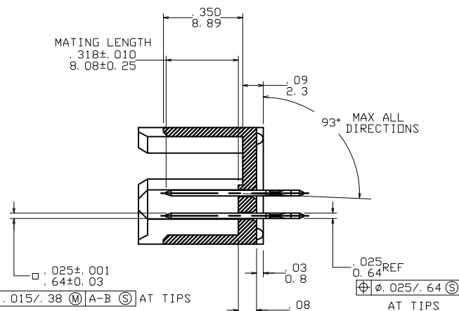
SECTION Y-Y
