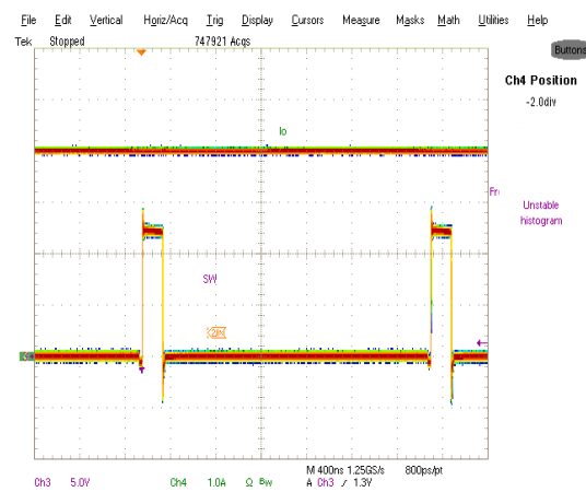
Fig. 18: Inductor node at 4A, sourcing current, Ch 3 :SW, Ch 4 :I out
