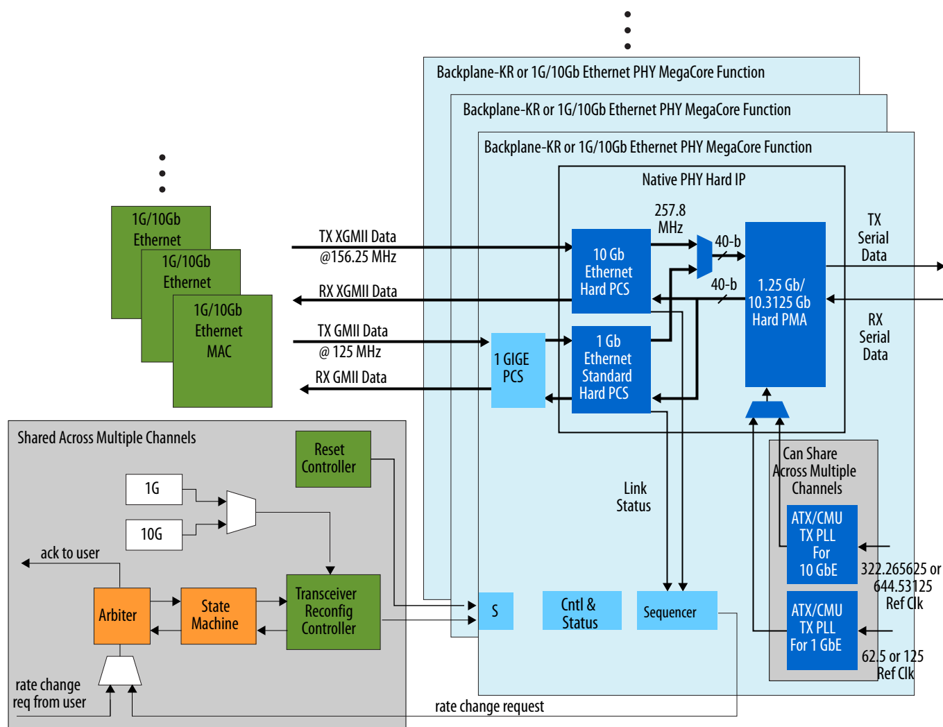
Figure 4-7: Block Diagram for Reconfiguration Example
