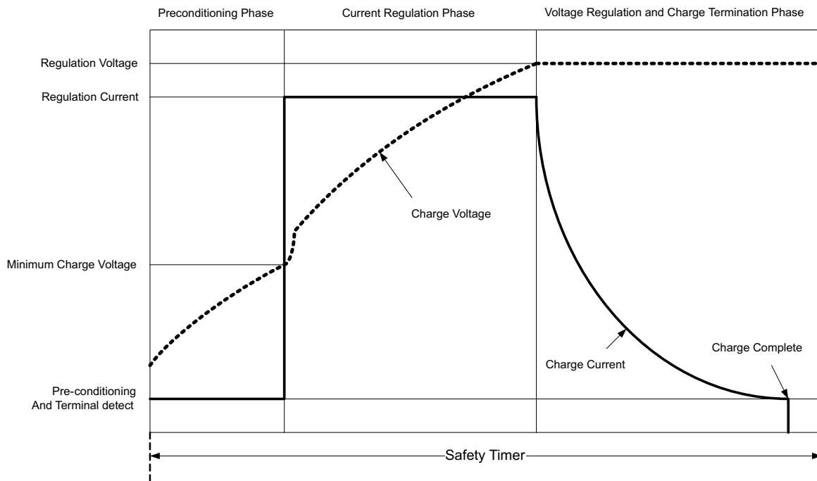
Figure 8. Charging Profile
