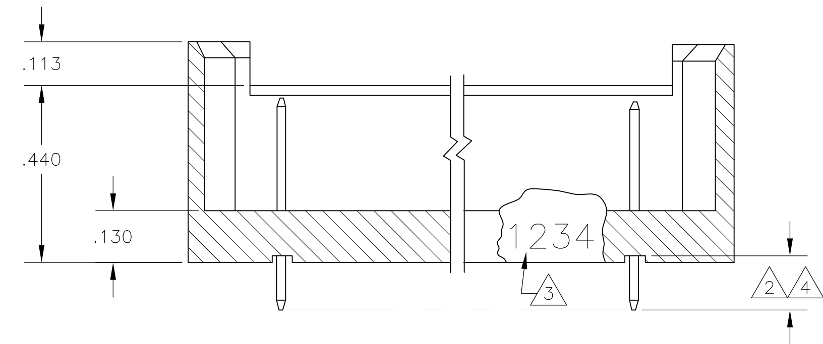
SECTION M-M
