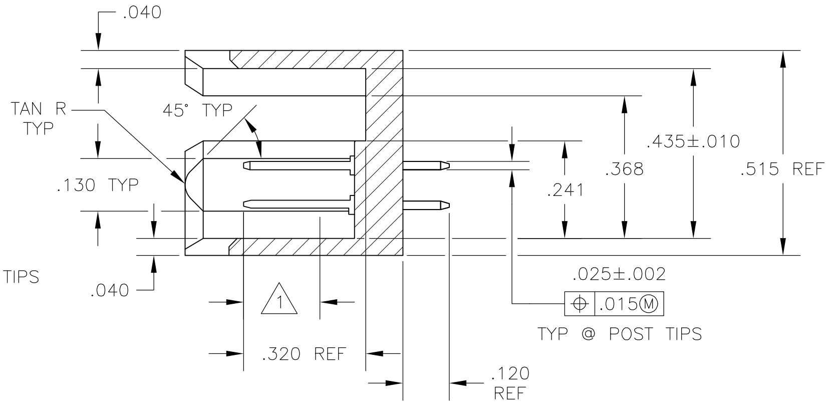
SECTION L-L
