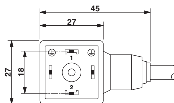
Dimensional drawing
