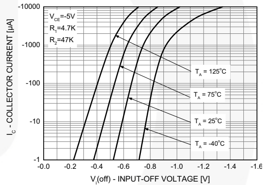
Figure 4. Input-Off Voltage
