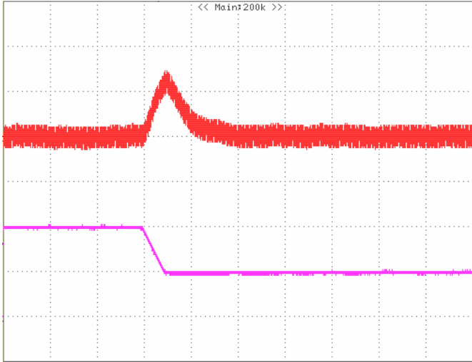
Figure 8: Output voltage response to step-change in load current (50%-25% of I_{o, max} ; di/dt = 0.1A/\mu s ). Load cap: 10\mu F , tantalum capacitor and 1\mu F ceramic capacitor. Top Trace: V_{out} (100mV/div, 100us/div), Bottom Trace: I_{out} (5A/div).
