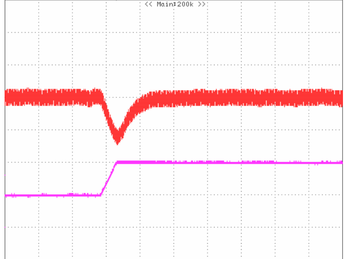
Figure 9: Output voltage response to step-change in load current (25%-50% of I_{o, max} ; di/dt = 0.1A/\mu s ). Load cap: 10\mu F , tantalum capacitor and 1\mu F ceramic capacitor. Top Trace: V_{out} (100mV/div, 10us/div), Bottom Trace: I_{out} (5A/div).
