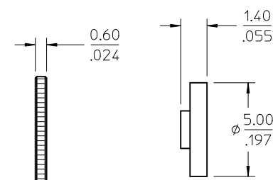
INSULATOR
