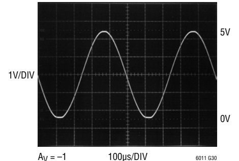
Rail-to-Rail Output Swing
