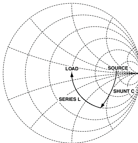
Figure 7. Smith Chart Representation of Step-Down Network
