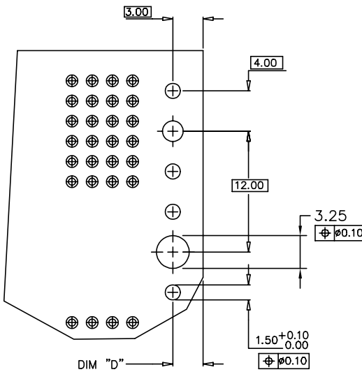
REQUIRED PC BOARD LAYOUT COMPONENT
