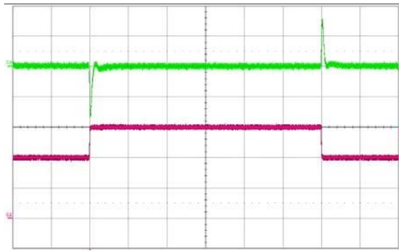
Figure 12. Output voltage response to load current step change (10A – 15A – 10A) at V_{\text{in}} = 48\text{V} . Top trace: output voltage (50mV/div.) Bottom: load current (5 A/div.). Current slew rate: 1 A/ \mu\text{s} . Time scale: 200 \mu\text{s} /div. C_{\text{o}} = 470\mu\text{F} POS + 1 \mu\text{F} ceramic
