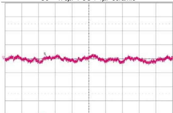
Figure 14. Input reflected-ripple current, is (10 mA/div.), measured through 10 \mu\text{H} at the source at full rated load current and V_{\text{in}} = 48\text{V} . Refer to Fig. J for test setup. Time scale: 1 \mu\text{s} /div.
