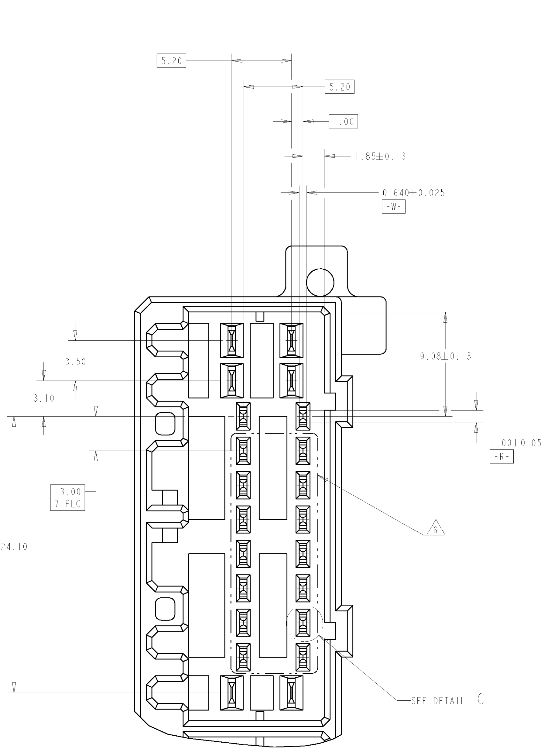
DETAIL E SCALE 5:1
