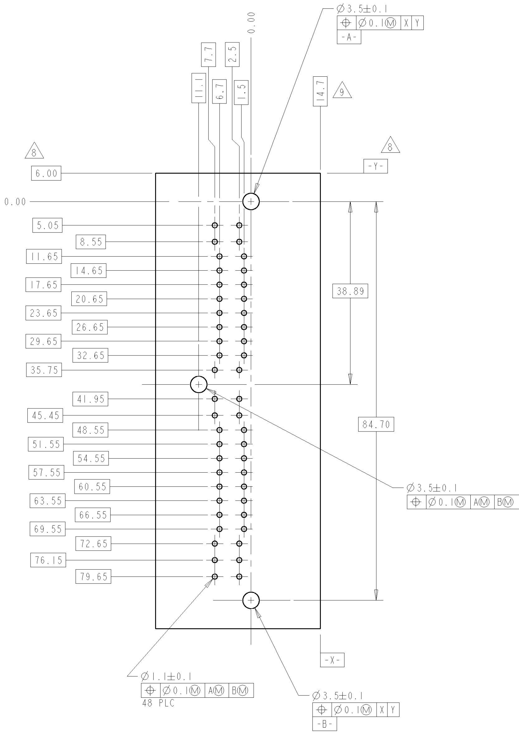
RECOMMENDED P.C. BOARD LAYOUT
