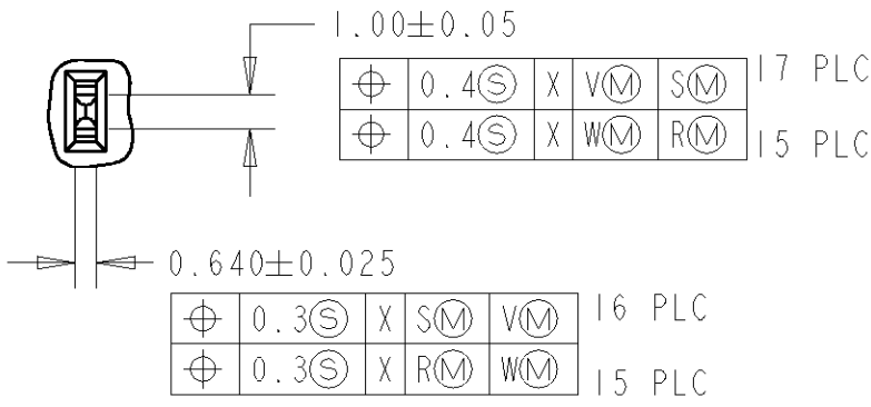
DETAIL C (.040 CONTACTS) SCALE 4:1
