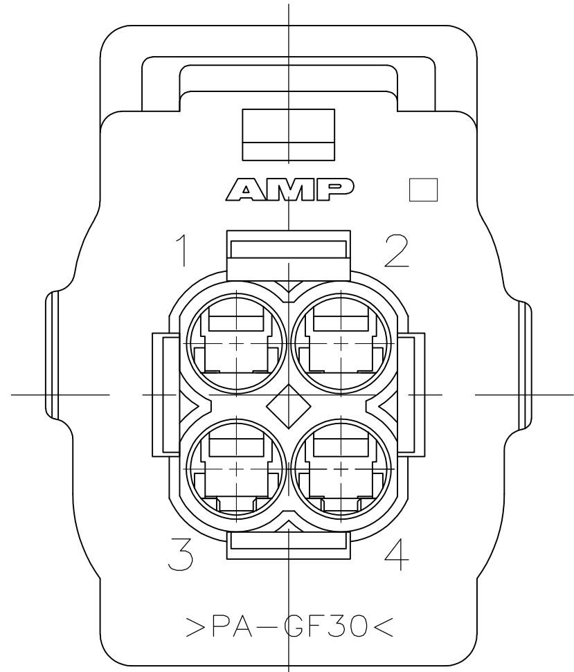
VIEW B-B
