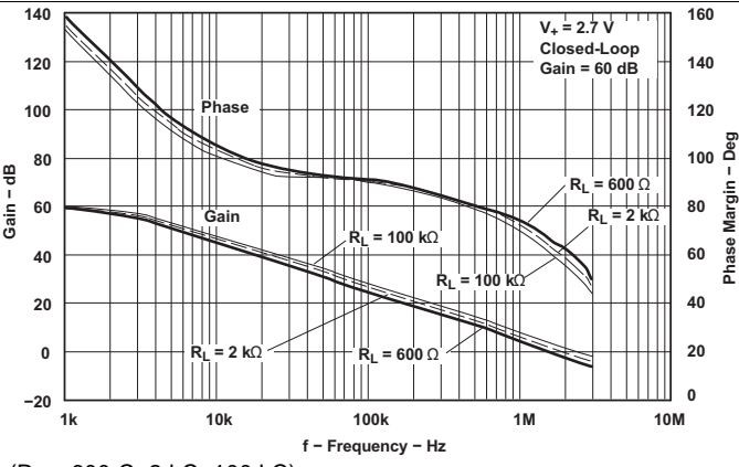
( R_L = 600 \Omega, 2 \text{ k}\Omega, 100 \text{ k}\Omega ) Figure 22. Gain and Phase Margin vs Frequency
