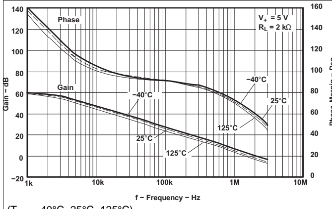
( T_A = -40^\circ\text{C}, 25^\circ\text{C}, 125^\circ\text{C} ) Figure 21. Gain and Phase Margin vs Frequency
