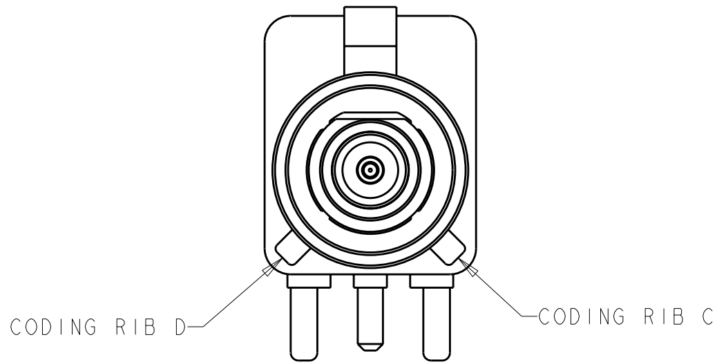
DETAIL K
