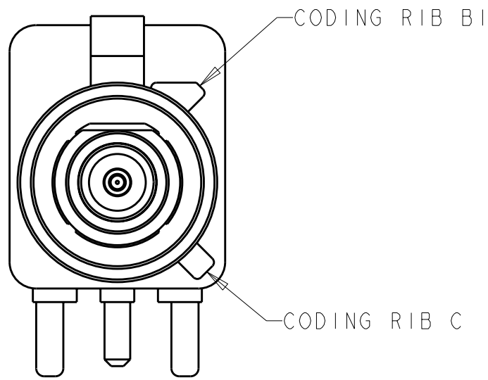
DETAIL F
