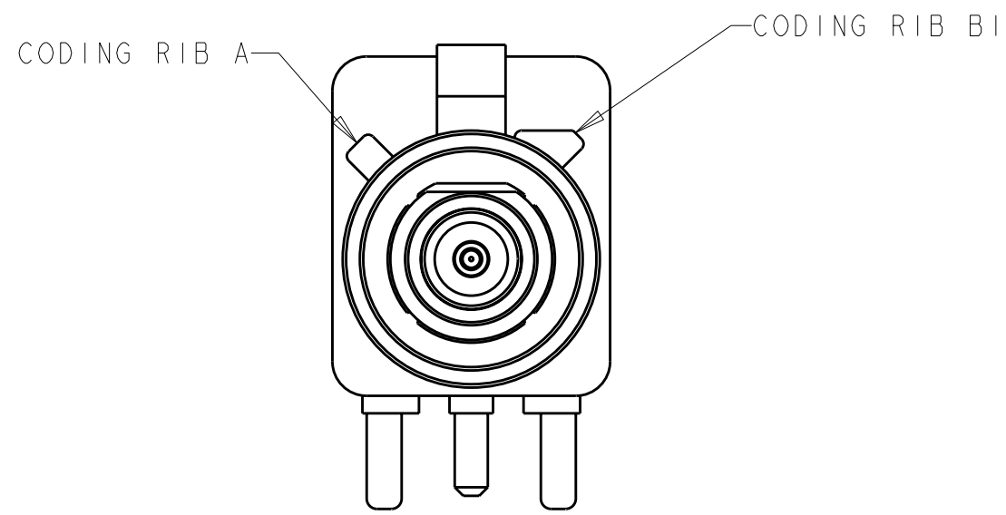
DETAIL A
