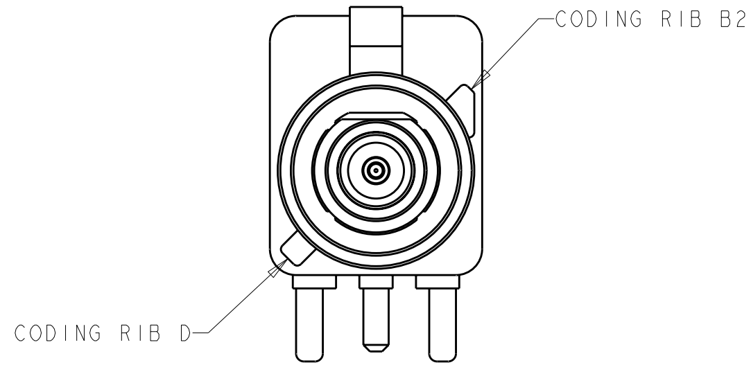
DETAIL I
