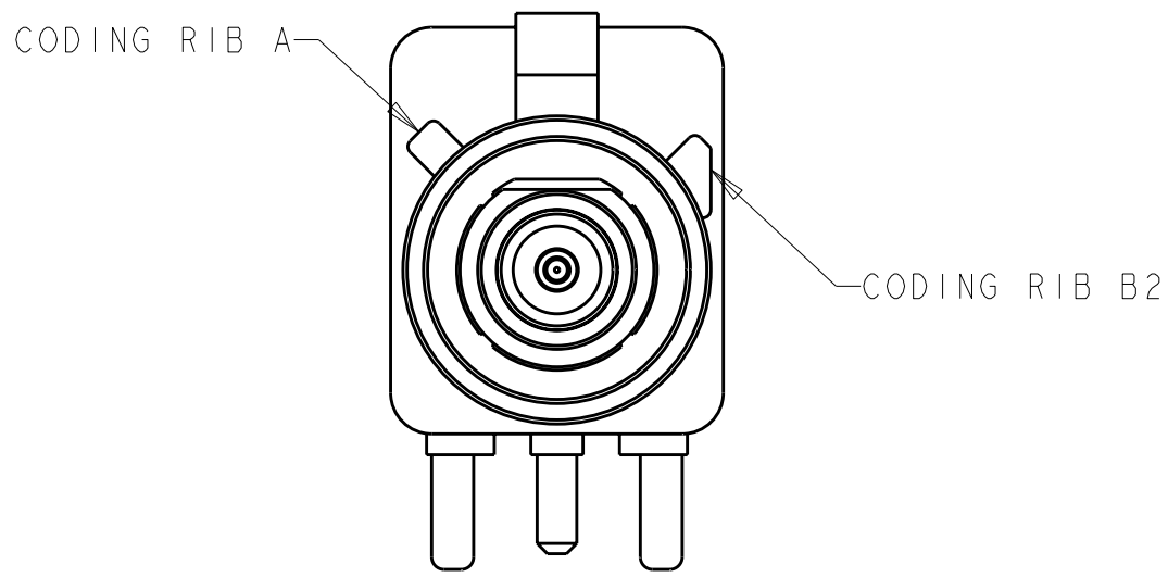
DETAIL B
