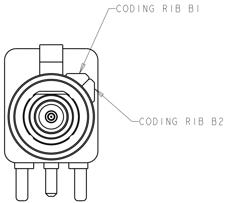
DETAIL E
