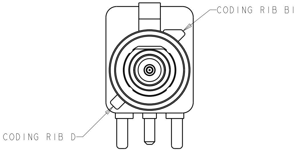
DETAIL G
