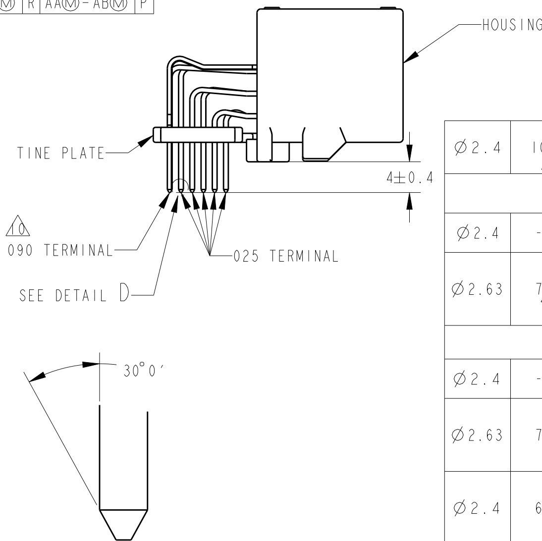
DETAIL D SCALE 20:1
