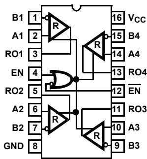
ISL32173E, ISL32273E (16 LD N-SOIC, 16 LD TSSOP) TOP VIEW
