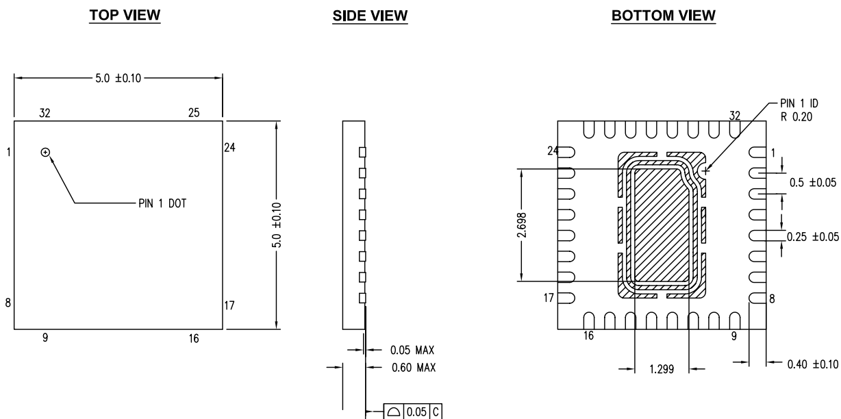
Figure 19. 32-Pin QFN 5 × 5 × 0.55 mm (Sawn)
