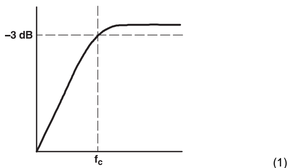
Figure 34. Input Resistor and Input Capacitor
