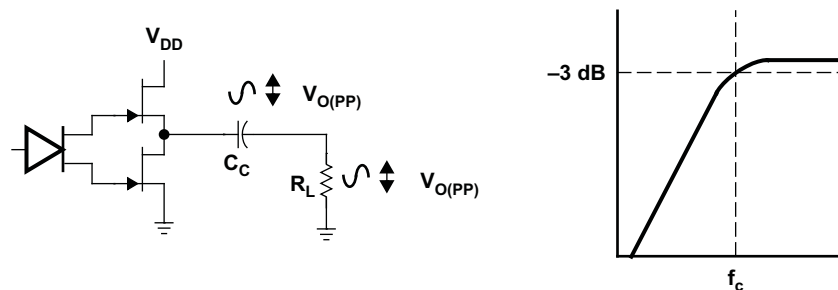
Figure 36. Single-Ended Configuration and Frequency Response
