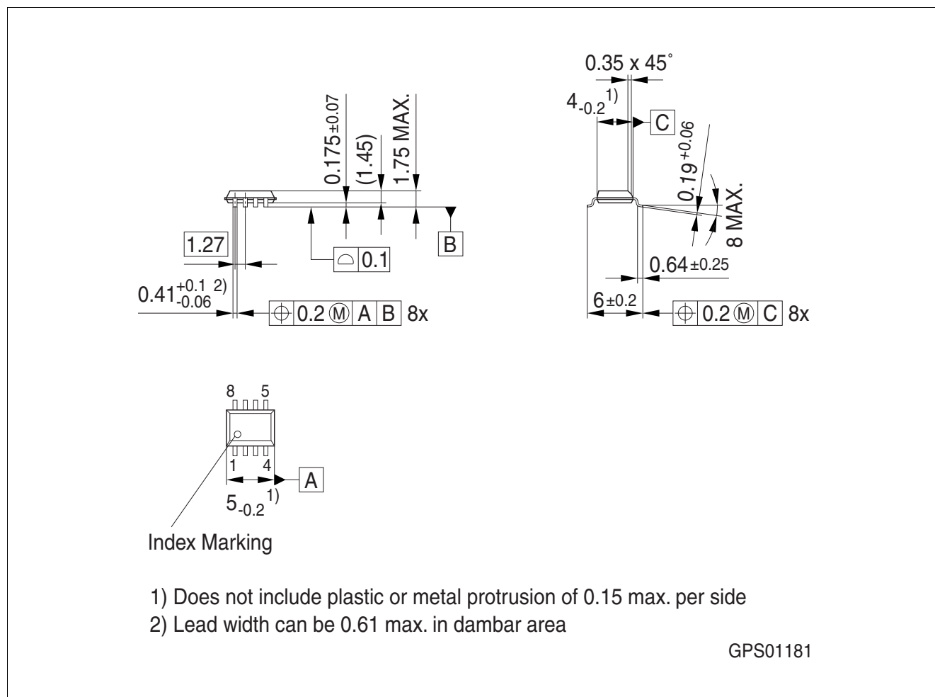
Figure 11 PG-DSO-8
