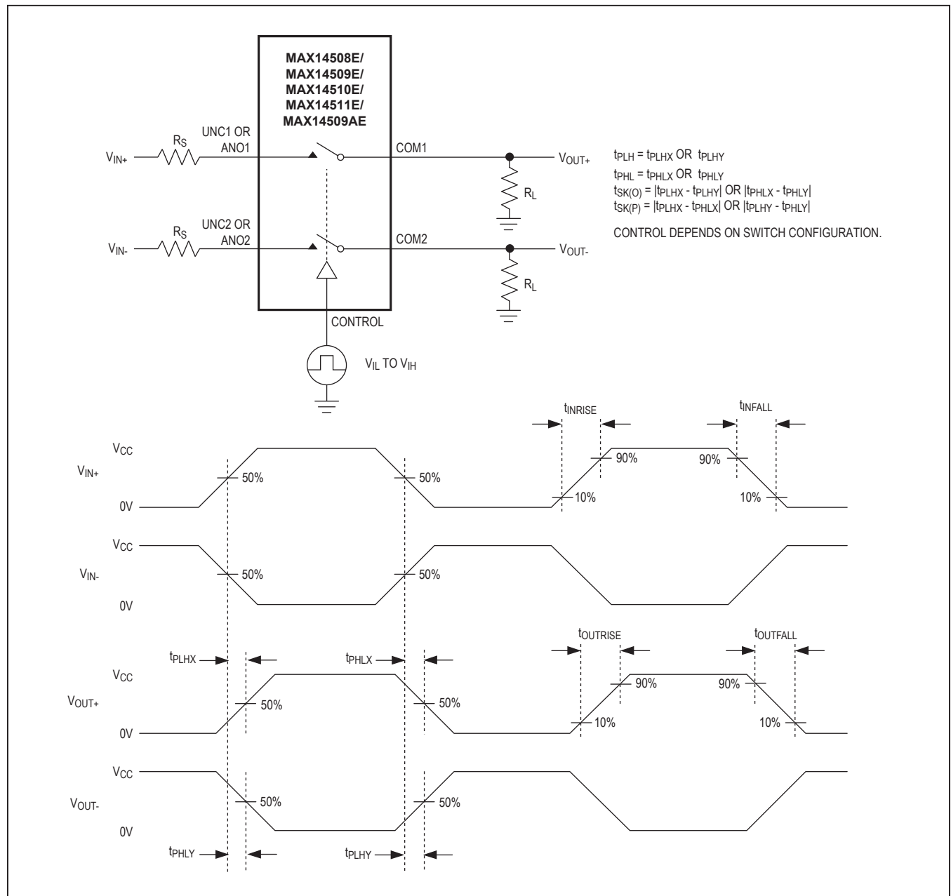
Figure 3. Output Skew
