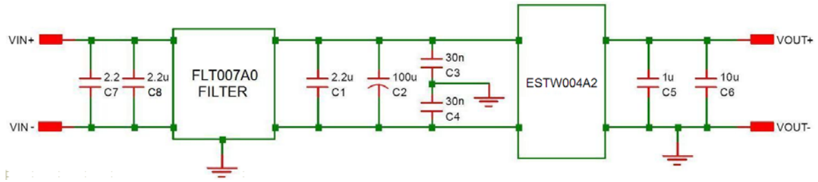
Figure 23. EMC Considerations
