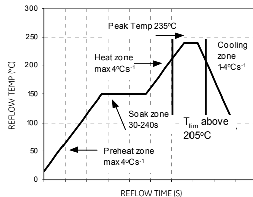
Figure 19. Reflow Profile for Tin/Lead (Sn/Pb) process
