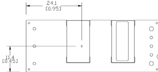
Figure 18. Pick and Place Location.
