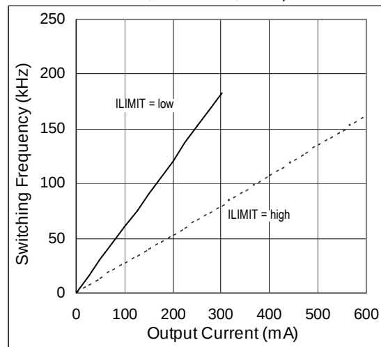
Figure 14. Switching Frequency vs. Output Current; V_{IN} = 12V, V_{OUT} = 3.3V, L = 10\mu H
