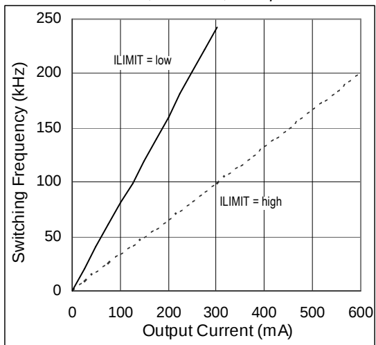
Figure 13. Switching Frequency vs. Output Current; V_{IN} = 12V, V_{OUT} = 5V, L = 10\mu H
