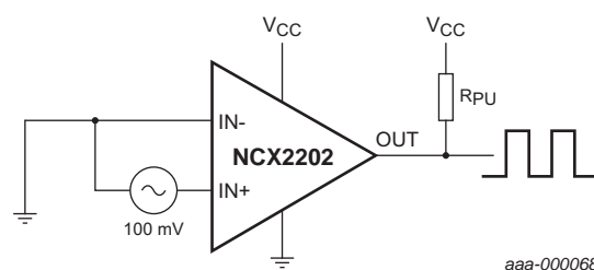
Fig 12. Zero-crossing detector
