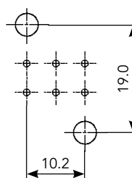
6 contacts
