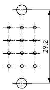
12 contacts
